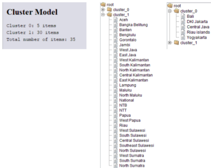
Figure 4. Final cluster results
